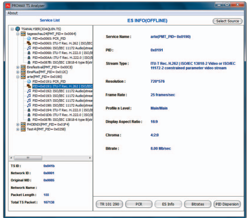
"Elementary Stream" information (independent audio or video stream contained into a TS)
