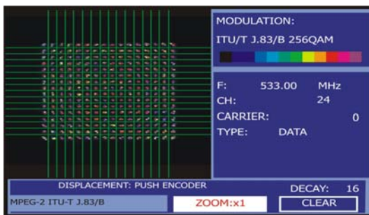
Figure 45.- Constellation Diagram. MPEG-2 TS ITU-T J.83/B.
