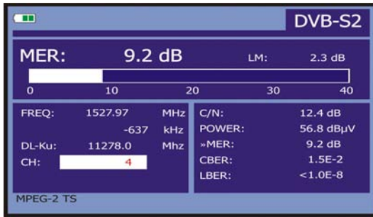
Figure 44.- DVB-S2 (QPSK/8PSK) signals MER measurement screen.
