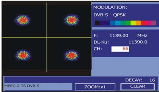
Figure 48.- Constellation Diagram. DVB-S (QPSK) signal.
