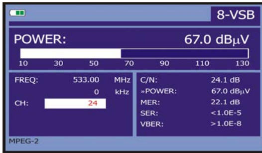
Figure 30.- Digital channel power measurement.
