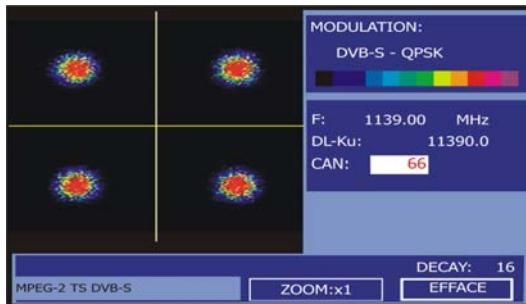
Figure 48.- Diagramme de constellation. Signal DVB-S (QPSK).
