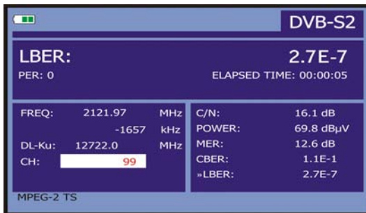
Figure 42.- DVB-S2 (QPSK/8PSK) signals LBER measurement screen.
