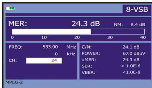
Figure 43.- Screen of MER measurement of ATSC (8-VSB) signals.
