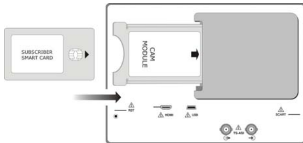
Figure 71.- Subscriber Smart-Card and CAM module insertion.
