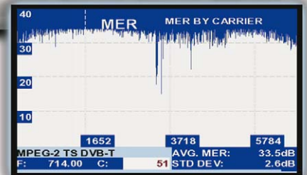
MER by carrier DVB-T (DVB-T2 optional)
