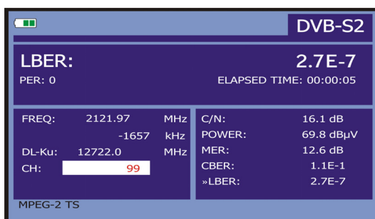
Figure 39.- DVB-S2 (QPSK/8PSK) signals LBER measurement screen.
