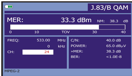
Figure 29.- Screen of BER measurement of QAM Annex-B signals.
