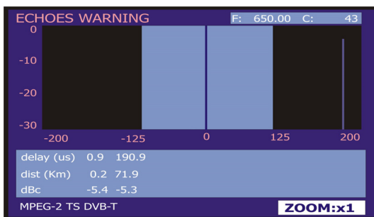
Figure 54.- ECHOES WARNING Screen.
