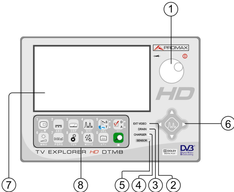
Figure 3.- Front panel.
