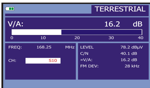
Figure 23.- Measurement of the video/audio ratio.
