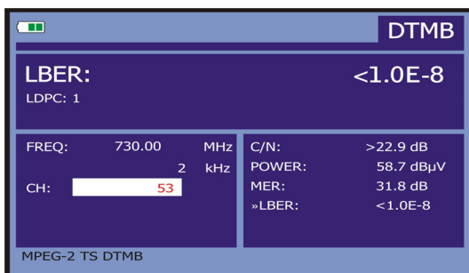
Figure 34.- DTMB signals LBER measurement screen.
