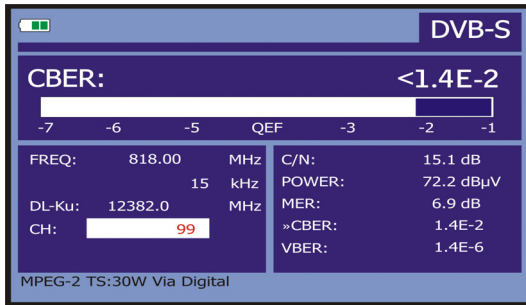
Figure 35.- DVB-S (QPSK) signals CBER measurement screen.
