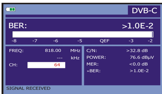
Figure 31.- DVB-C (QAM) signals BER measurement screen.
