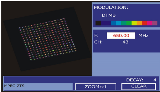
Figure 44.- Constellation Diagram. DTMB (QAM 256) signal.
