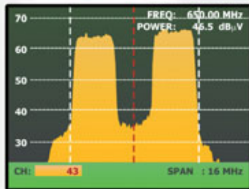
Spectrum hole unveiling the presence of intermodulation products within the channel
