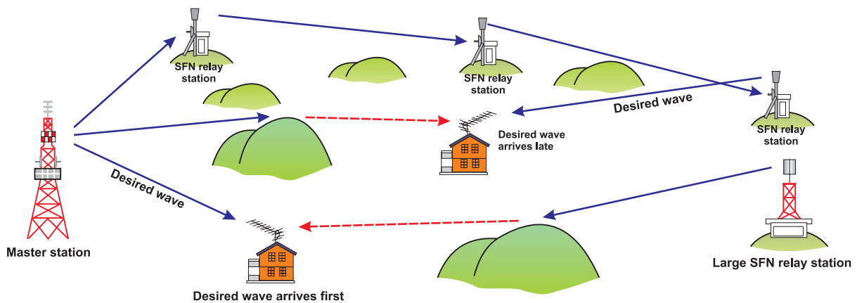
Multipath interference outside the guard interval in digital terrestrial broadcasting
